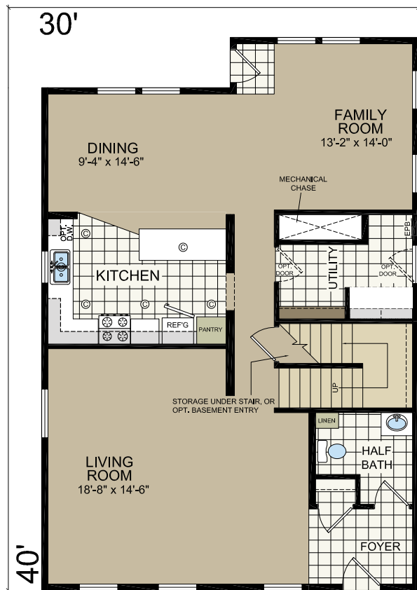
1ST FLOOR
