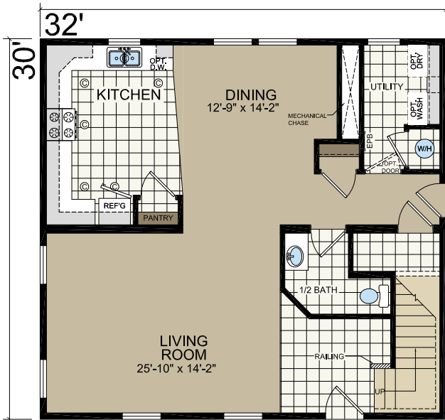
1ST FLOOR
