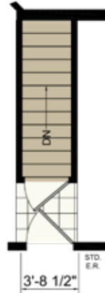
OPTION STAIRWELL
