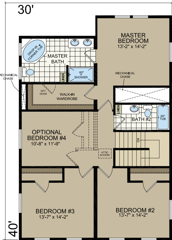
2nd FLOOR
