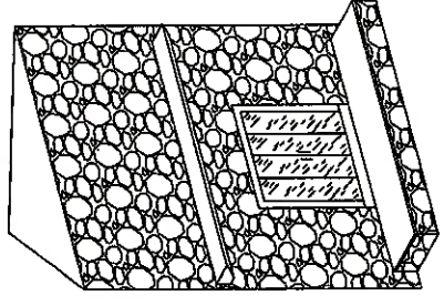
109 CORNER RAISED HEARTH FIREPLACE w/ FULL STONE SURROUND
