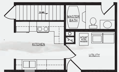
BASEMENT PLAN
