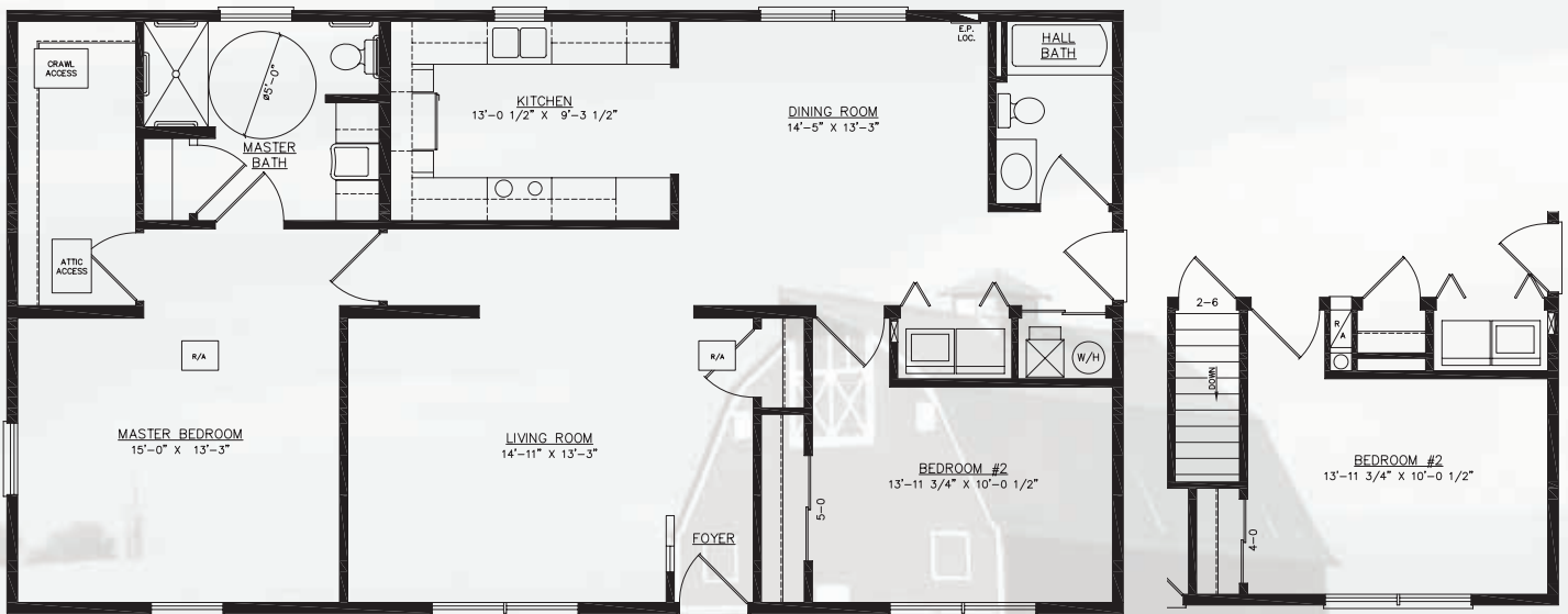
CRAWLSPACE PLAN
