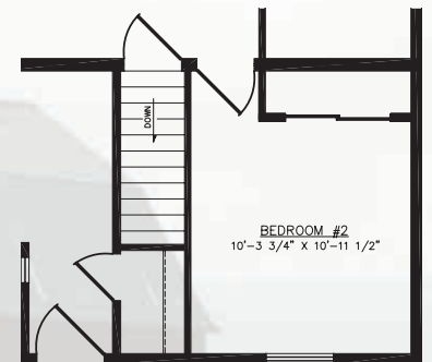
BASEMENT PLAN
