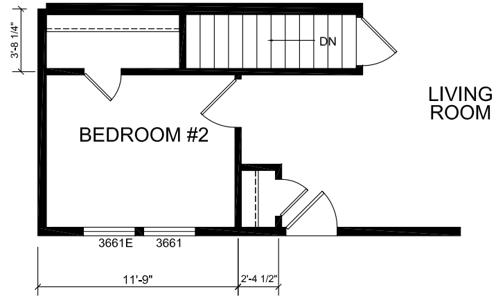
STAIRWELL OPTION
