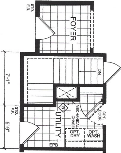
OPTIONAL STAIRWELL * (FURNACE, W/H & WARM AIR DUCTS ON-SITE BY OTHERS)
